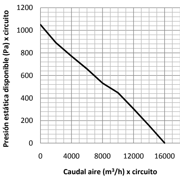
ETCB/F-45.1 - 90.2
