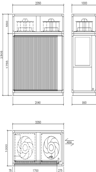
ETCB 70.1
