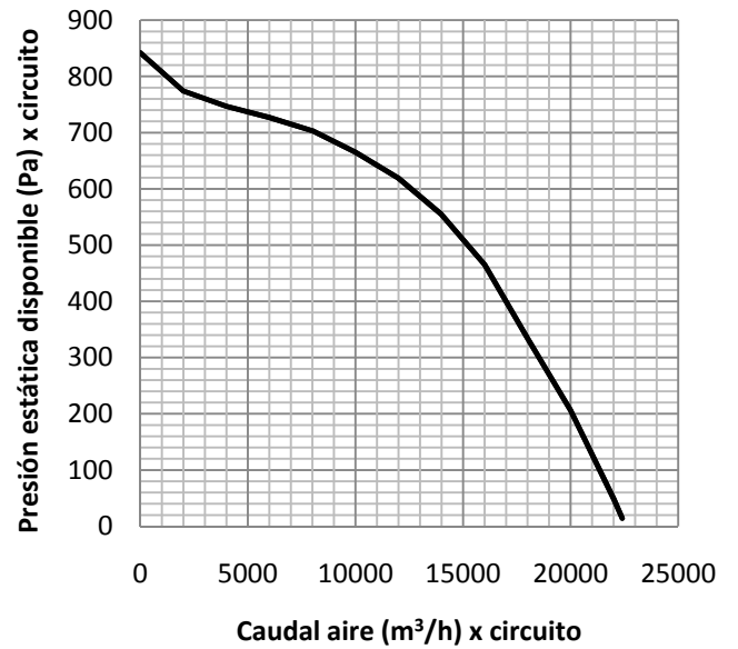
ETCB/F-255.3 - 340.4
