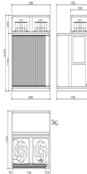
ETCB 70.1+DI
