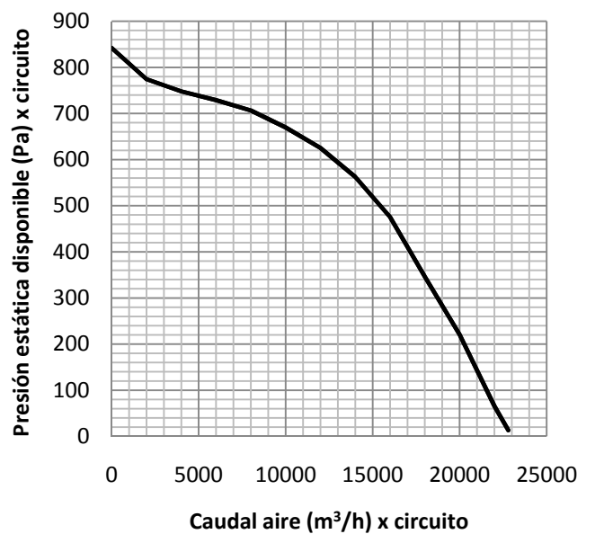
ETCB/F-60.1 - 120.2 - 180.3 - 230.4
