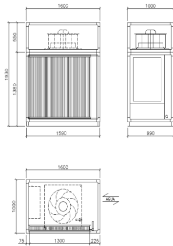
ETCB 30.1-40.1
