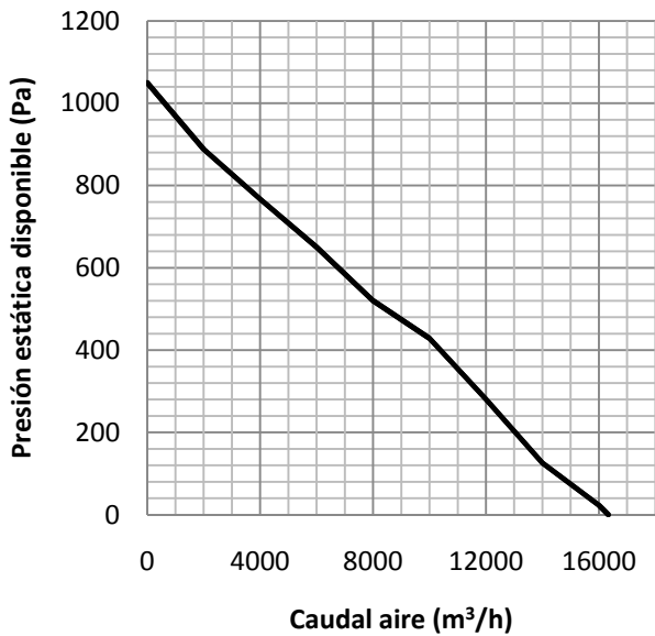
ETCB/F-30.1
