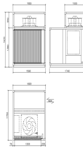
ETCB 30.1-40.1 +DI
