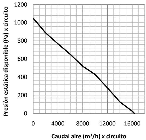
ETCB/F-40.1 - 80.2
